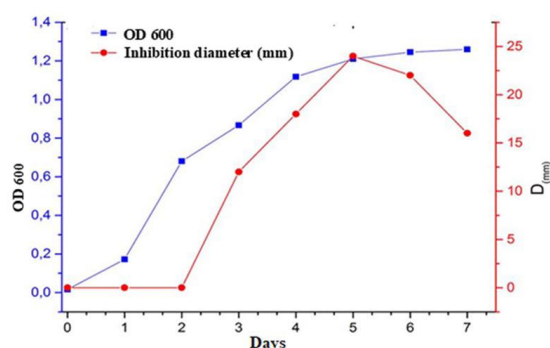
Fig. 3. Halopiger djelfimassiliensis G3A cell growth and antimicrobial production against the target strain Halorubrum saccharovorum AMR1.
