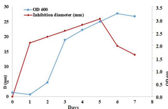
Fig. 4. Natrialba aegyptia TSA4 cell growth and antimicrobial production against the target strain Halorubrum terrestre AMB1.
