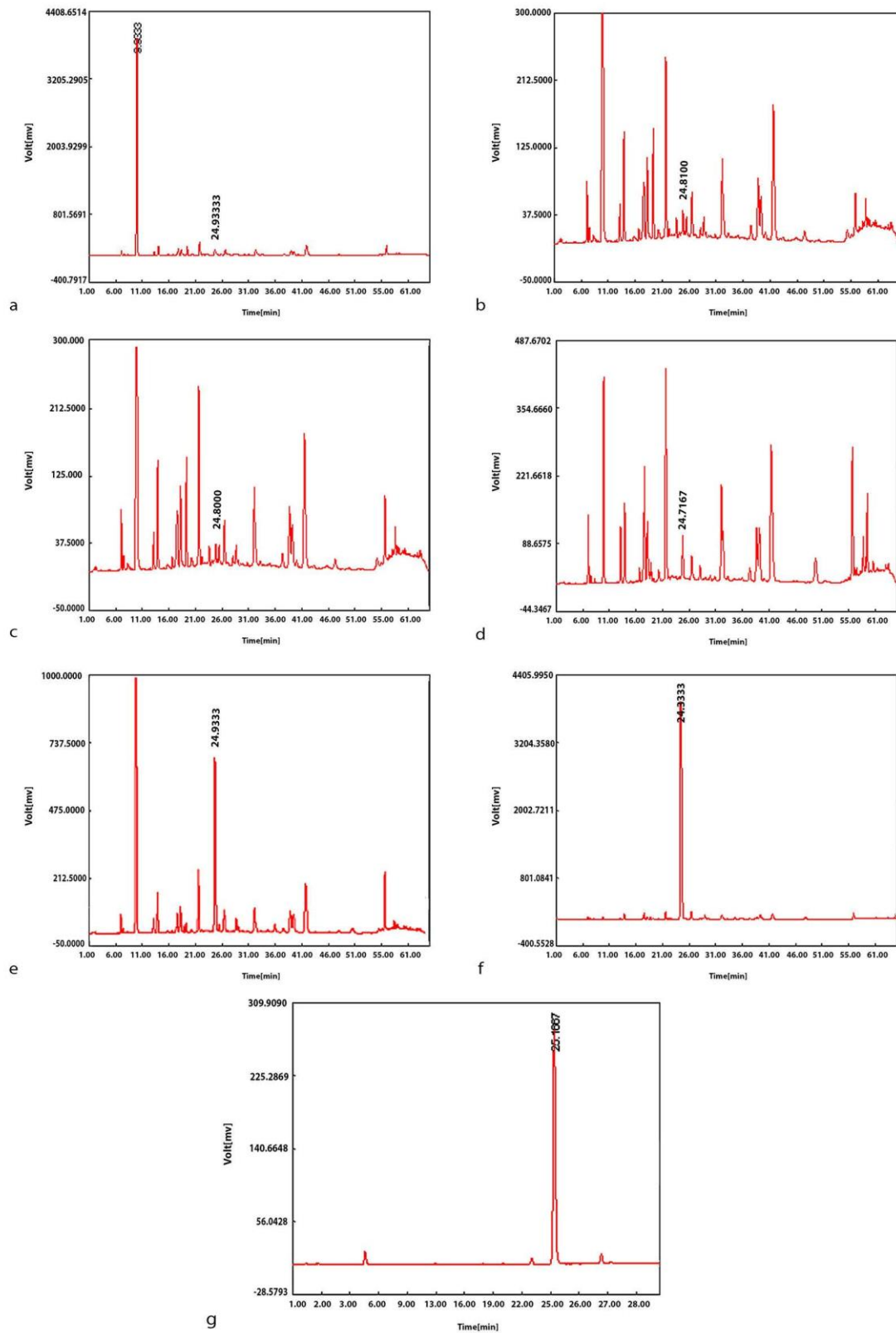
Fig. 1. Chromatogram of GABA production by lactic acid bacteria in MRS broth, a) Lactobacillus. delbrukii bulgaricus , b) Lactobacillus. rhamnosus c) Lactobacillus.casei d) Steteptocoos. thermophilos e) Lactococcus lactis. lactis f) Lactobacil- lus. Brevis g) standard sample
